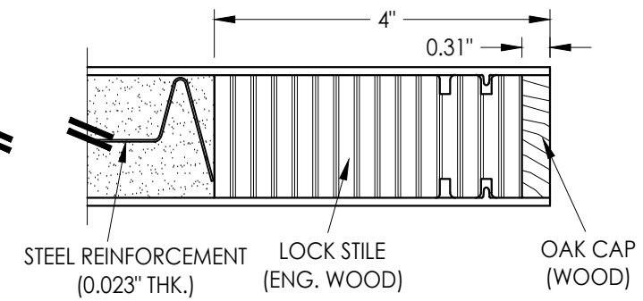
2 2 HORIZONTAL CROSS SECTION
